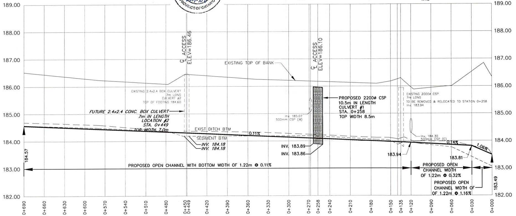
OUTLET DETAIL NTS
