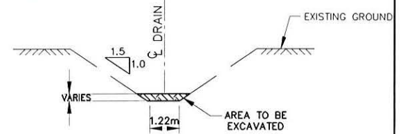
TYPICAL DRAIN CROSS SECTION (STA. 0+000 TO 1+265) NTS
