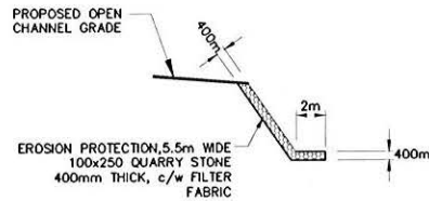
OUTLET DETAIL NTS
