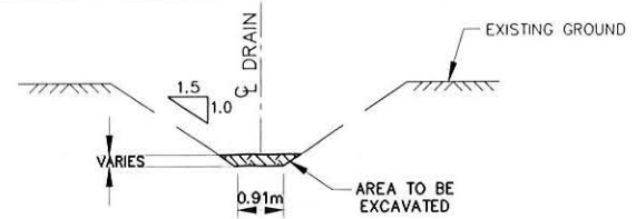
TYPICAL DRAIN CROSS SECTION (STA. 1+265 TO 3+780) NTS
