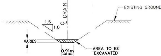
TYPICAL DRAIN CROSS SECTION (STA. 1+265 TO 3+780) NTS
