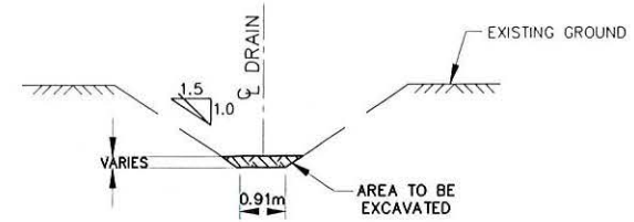
TYPICAL DRAIN CROSS SECTION (STA. 4+000 TO 4+990) NTS
