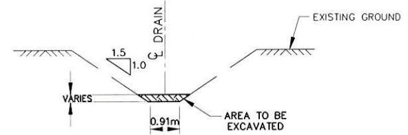
TYPICAL DRAIN CROSS SECTION (STA. 1+265 TO 3+780) NTS
