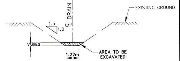
TYPICAL DRAIN CROSS SECTION (STA. 0+000 TO 1+265) NTS
