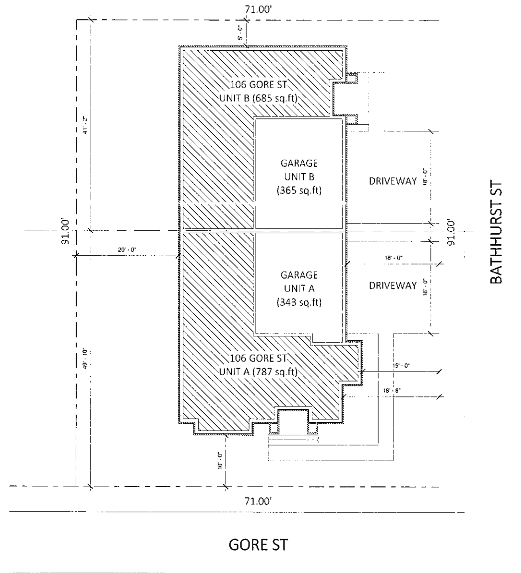
1 Proposed Site Plan 1/8" = 1'-0"
