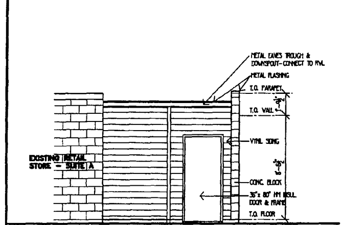
NEW RETAIL ADDITION - SUITE B REAR ELEVATION SCALE 1/4" = 1'-0"
