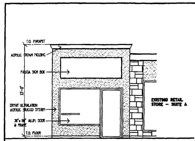
NEW RETAIL ADDITION - SUITE B FRONT ELEVATION SCALE 1/4" = 1'-0"
