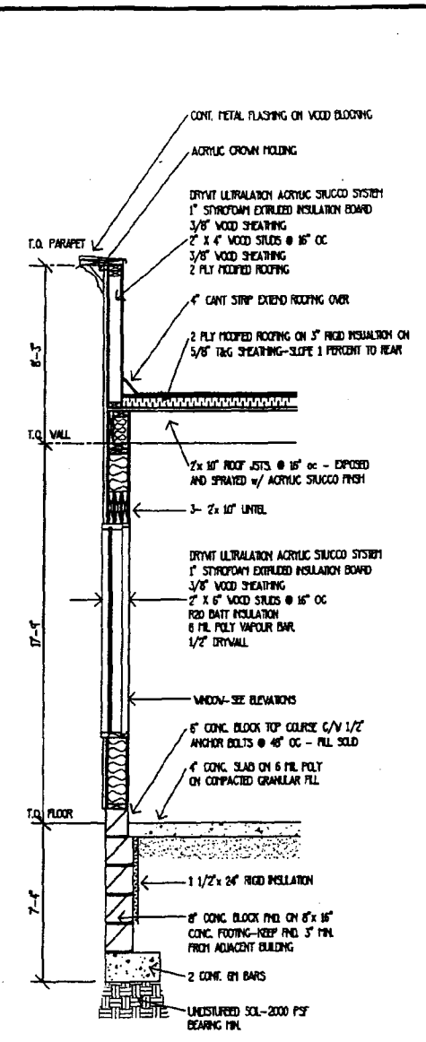
B WALL SECTION SCALE 1/2" = 1'-0"
