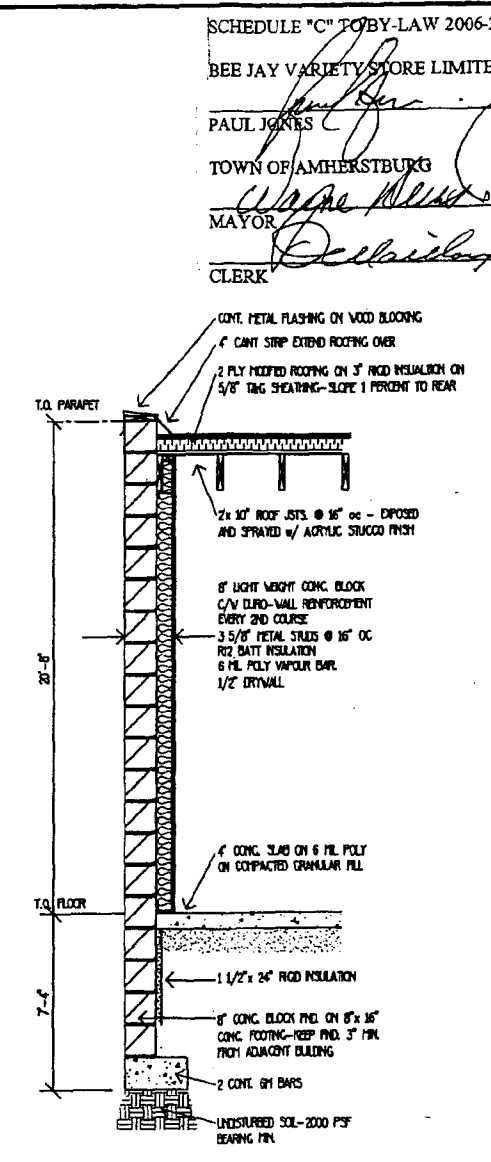
A WALL SECTION SCALE 1/2" = 1'-0"
